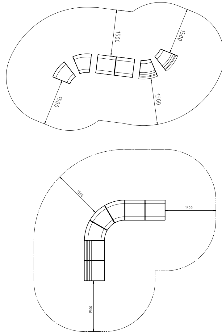
Diagram 4: Possibility of Installation
